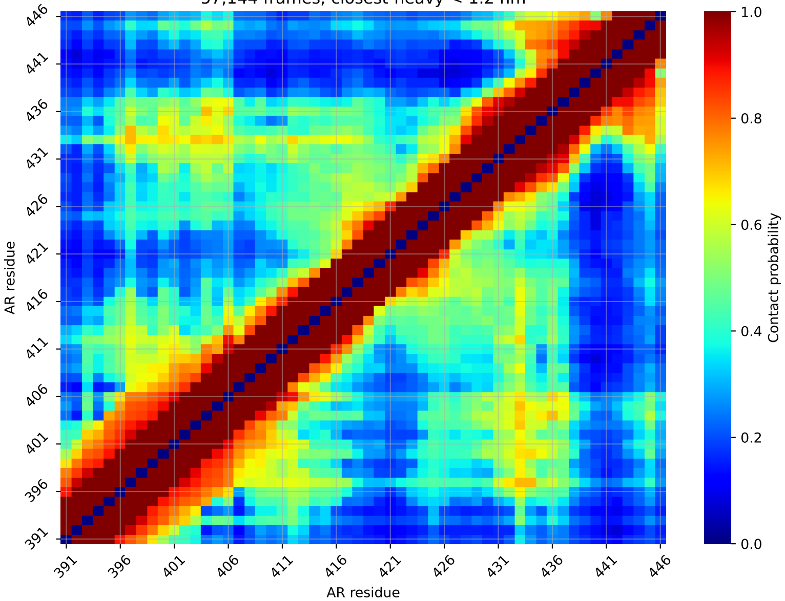
2022 apo WT MD — AR391-446 57,144 frames; closest-heavy < 1.2 nm
