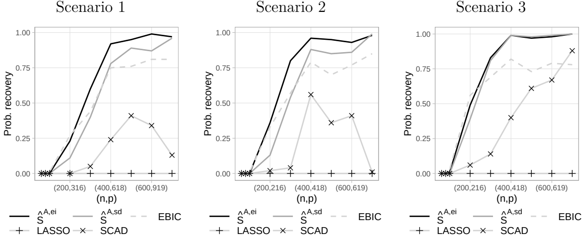
Figure 1: Probability of correct selection with externally-informed \hat{S}^{A,ei} , non-informed \hat{S}^{A,sd} , EBIC, LASSO and SCAD in Scenario 1 (left), 2 (middle), 3 (right).
