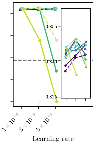
Full LoRA
