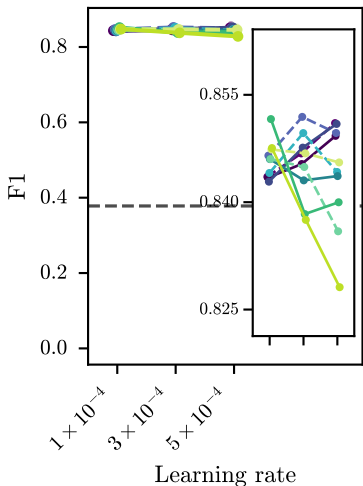
Query-Value LoRA
