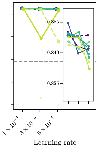
Attention LoRA
