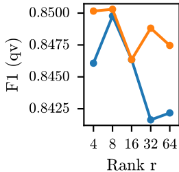
SQuAD
