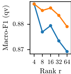
MNLI
