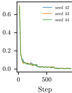
Attention LoRA
