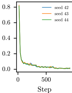
Query-Value LoRA
