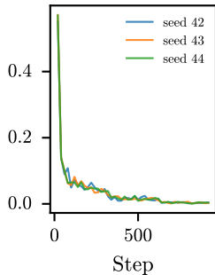
Full LoRA
