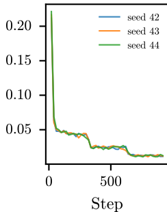
Attention LoRA
