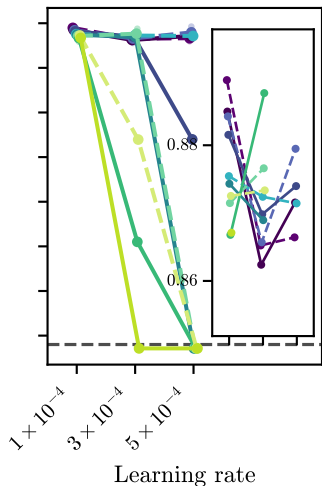
Full LoRA
