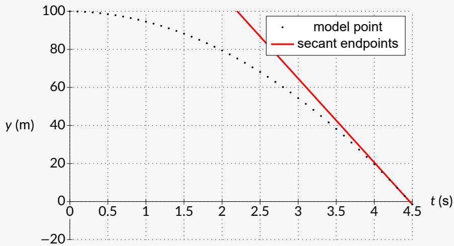
Figure 3: y(t) -diagram
