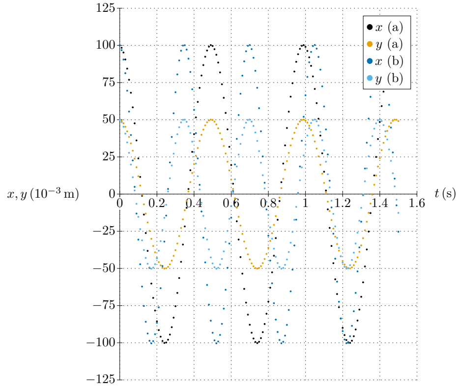
Figure 4: x, y(t) -diagram
