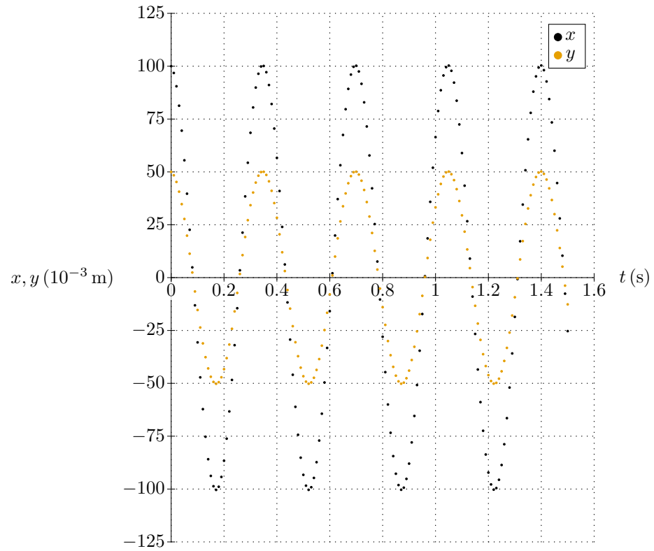
Figure 2: x, y(t) -diagram
