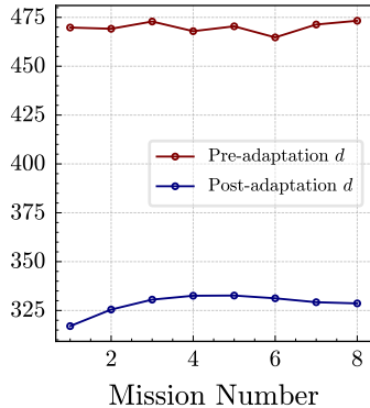
Subspace Distance d
