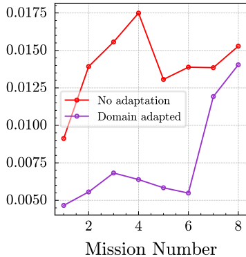
RMSE
