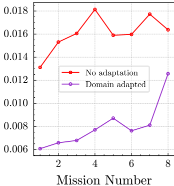
RMSE
