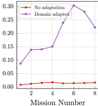
RMSE
