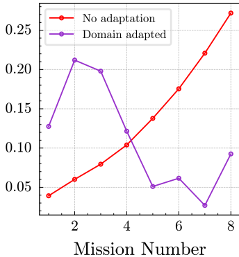
RMSE
