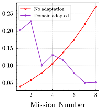
RMSE
