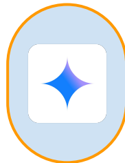
Gemini 2.5 Flash-Lite
