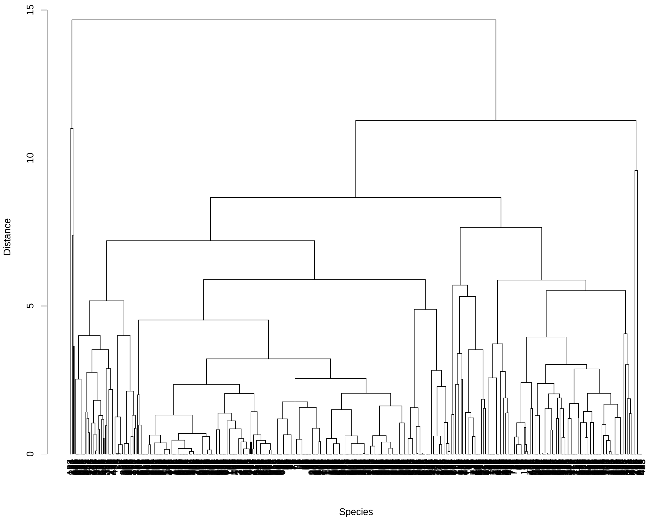
Dendrogram for 97 Species
