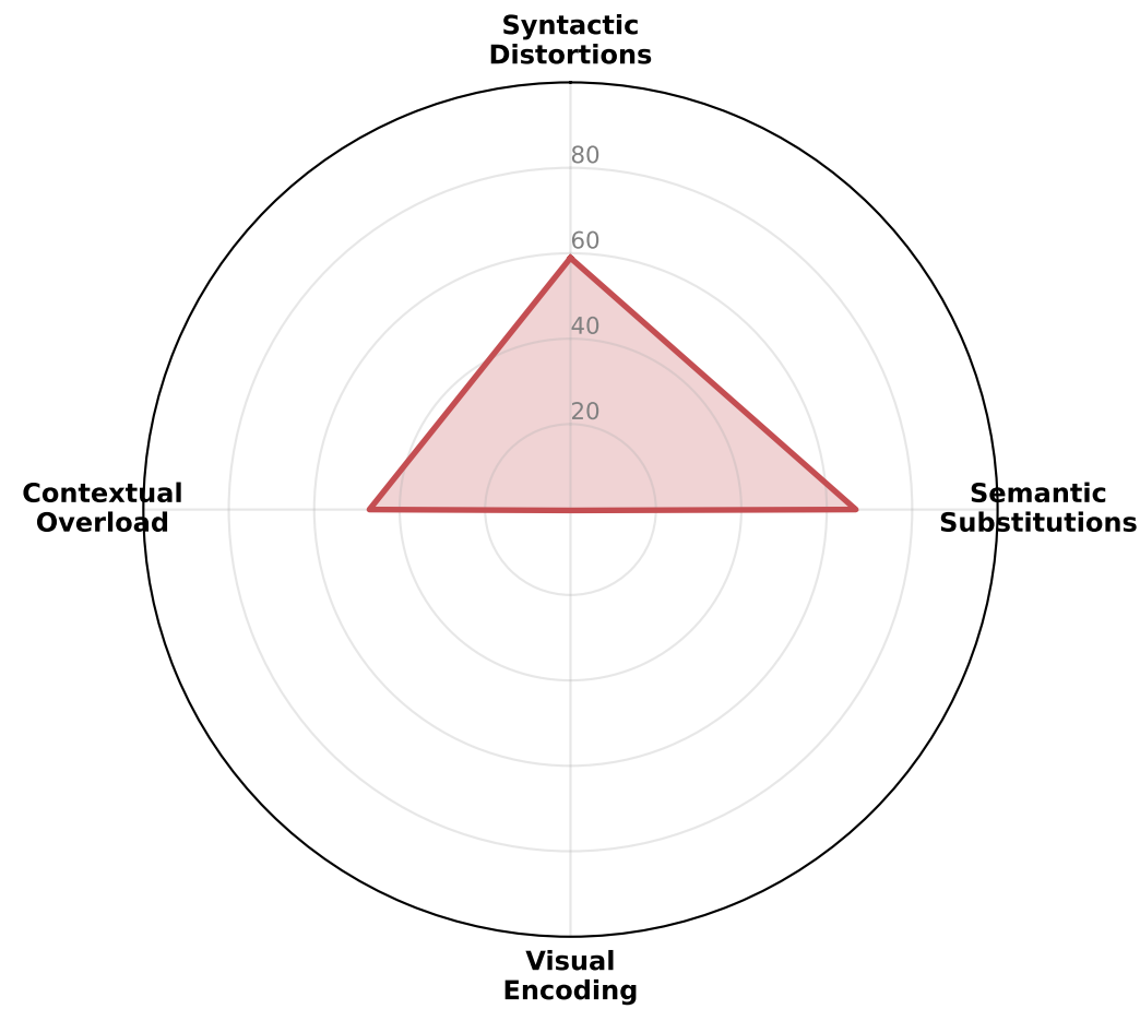
DSR1-Llama-70B
