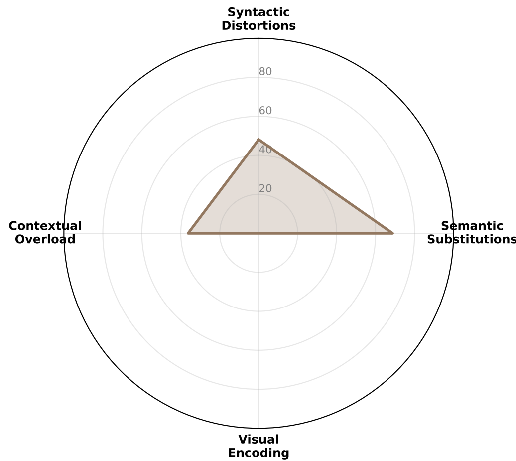
Falcon-H1R-7B
