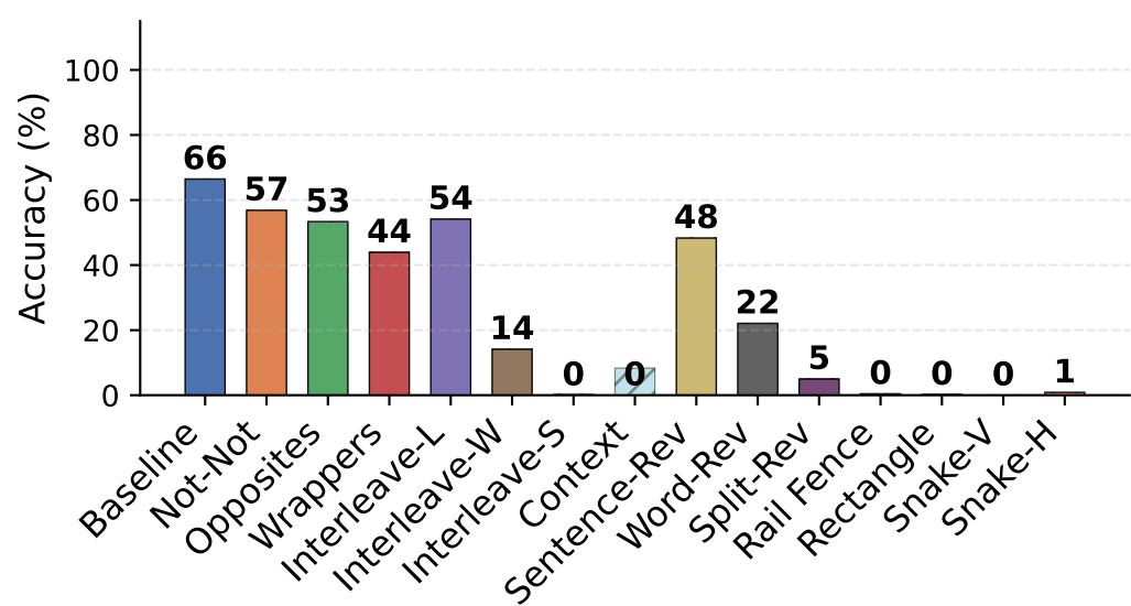
DSR1-Llama-70B
