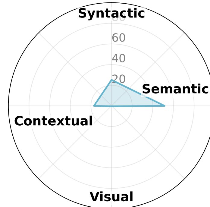
DSR1-Llama-70B
