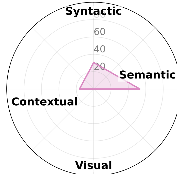
Nemotron-7B
