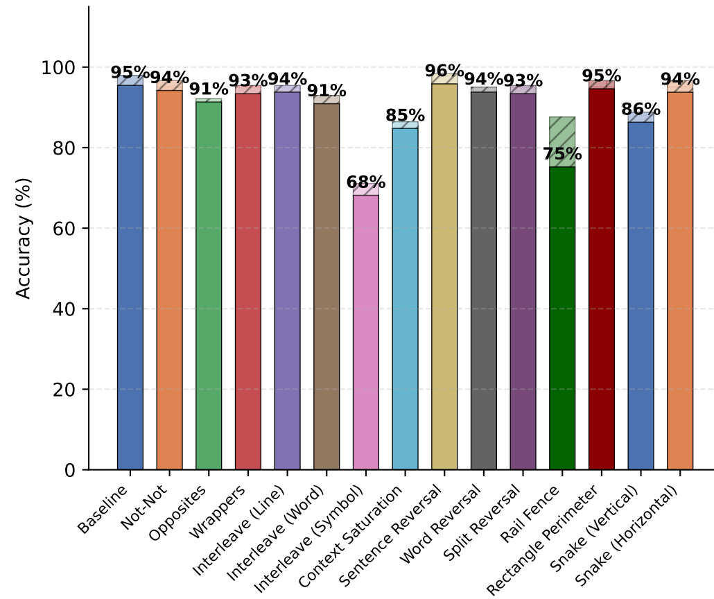
Falcon-H1R-7B
