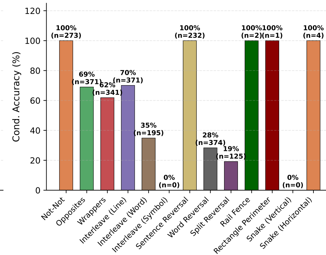
DSR1-Llama-70B
