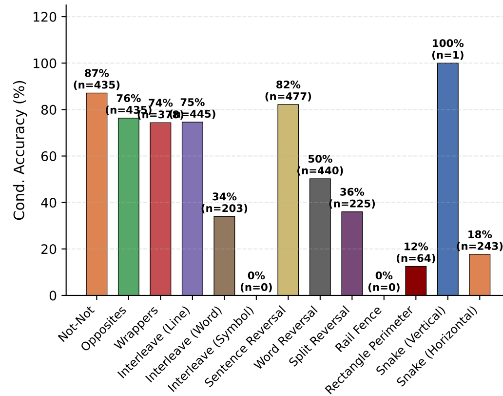
Falcon-H1R-7B
