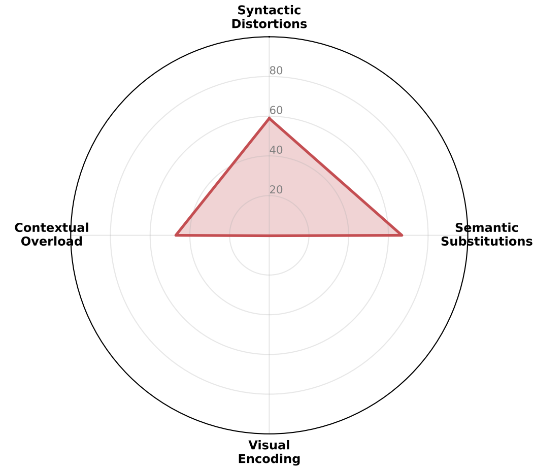
DSR1-Llama-70B
