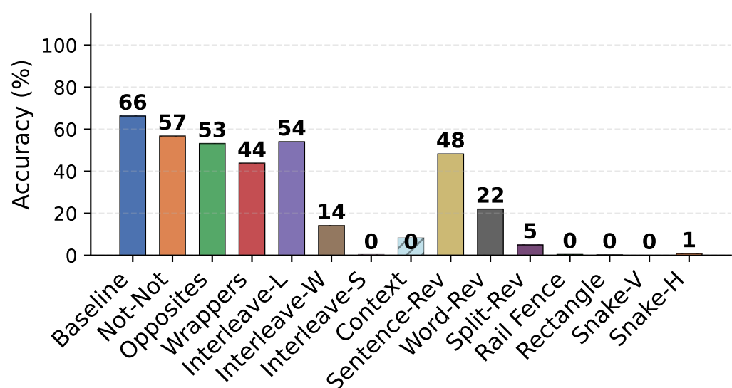
DSR1-Llama-70B
