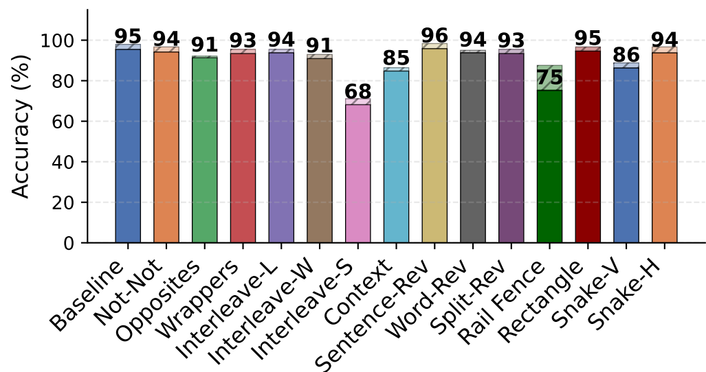
GPT-OSS-120B
