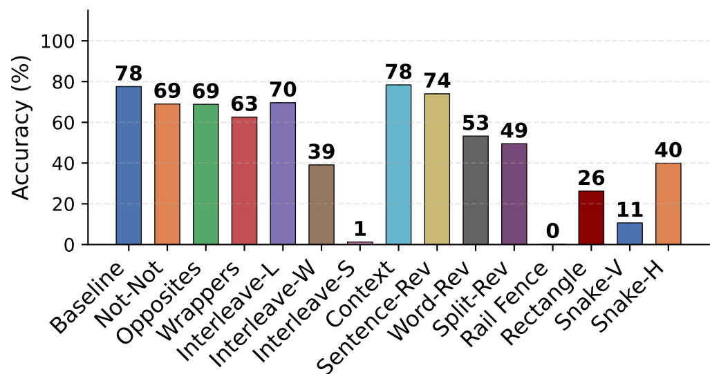
Falcon-H1R-7B
