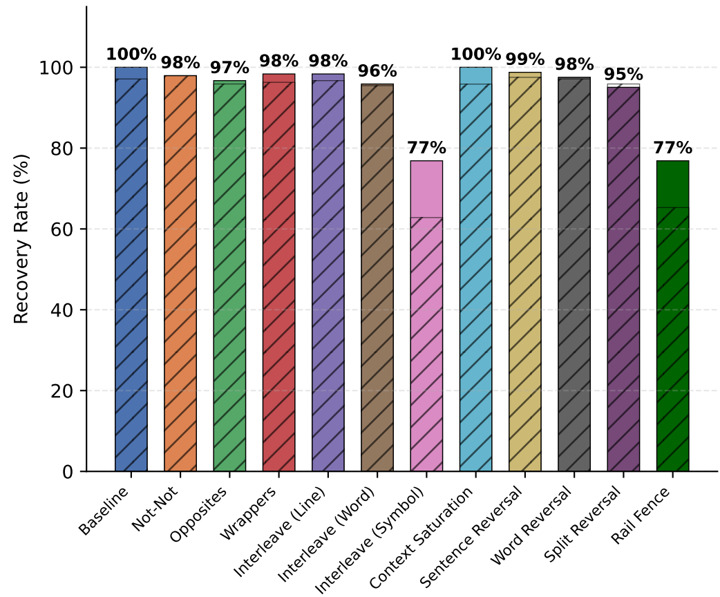
GPT-OSS-120B
