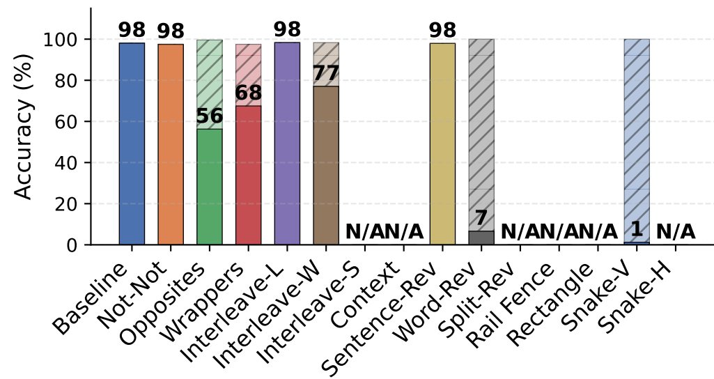
GPT-OSS-120B
