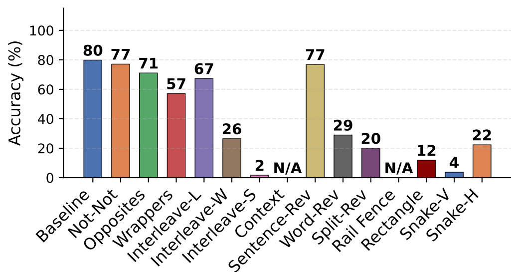
DSR1-Llama-70B
