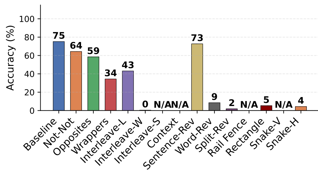
Nemotron-7B
