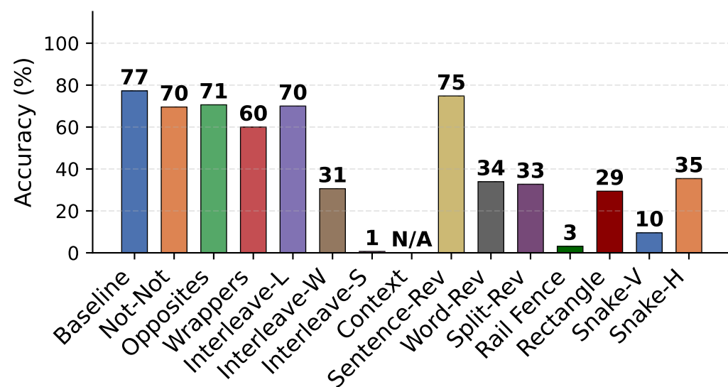
Nemotron-7B
