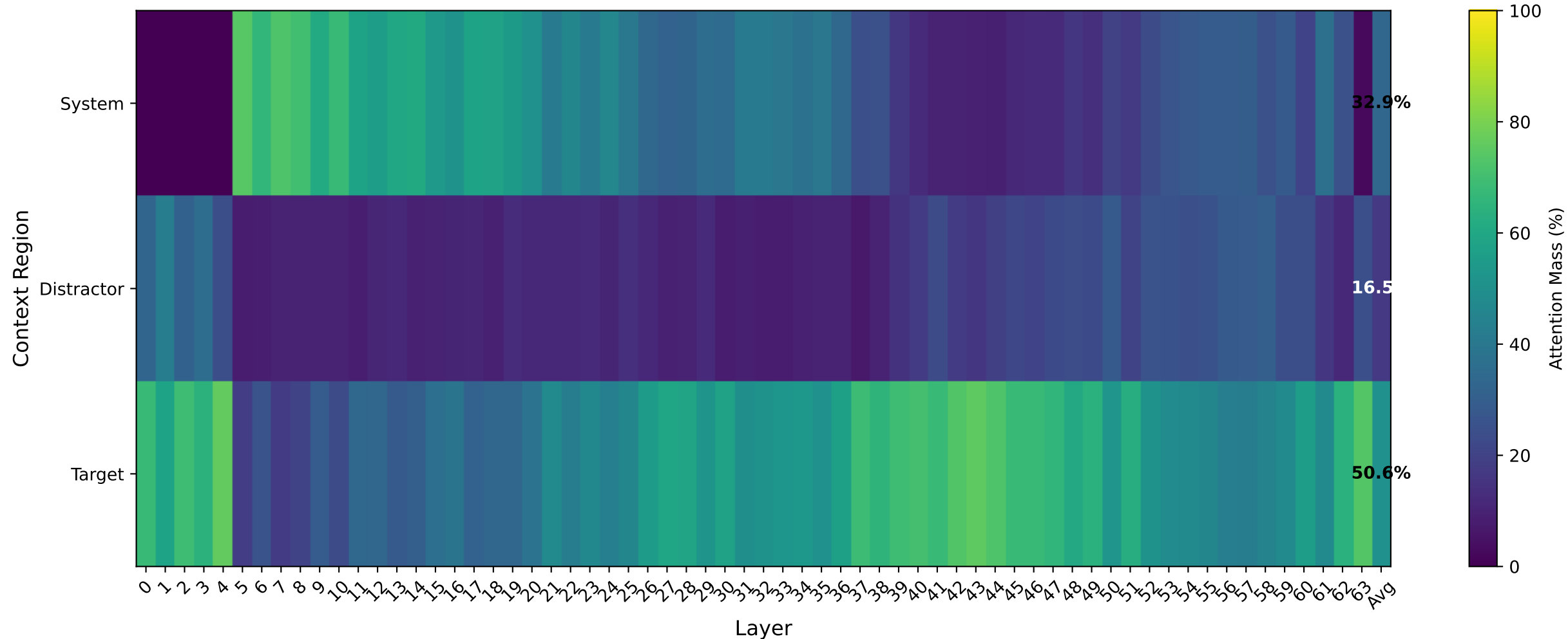
Attention Dilution: nvidia_OpenReasoning-Nemotron-32B (Run Date: 20260406_102432)
