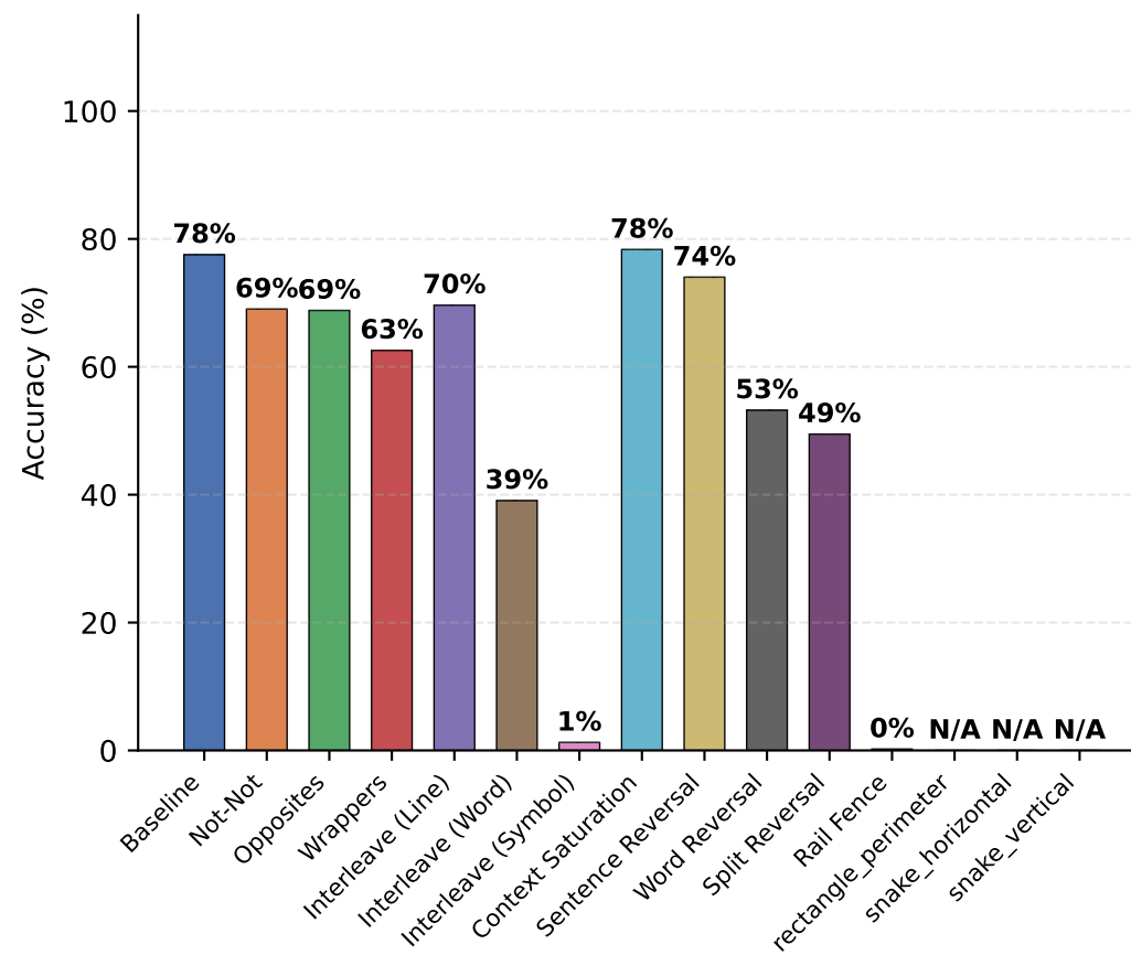
GPT-OSS-120B
