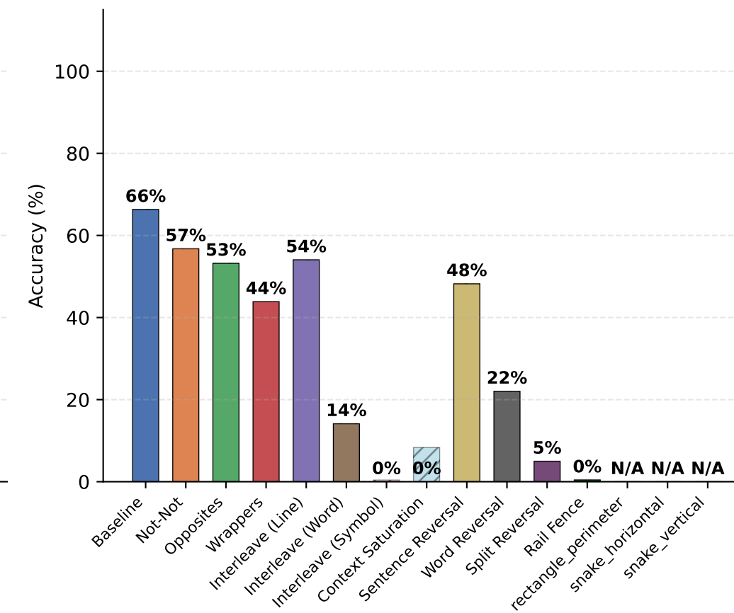
DSR1-Llama-70B
