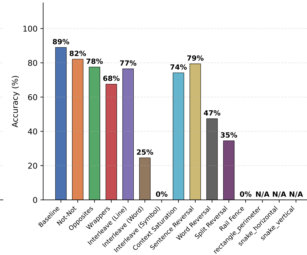
DSR1-Llama-70B
