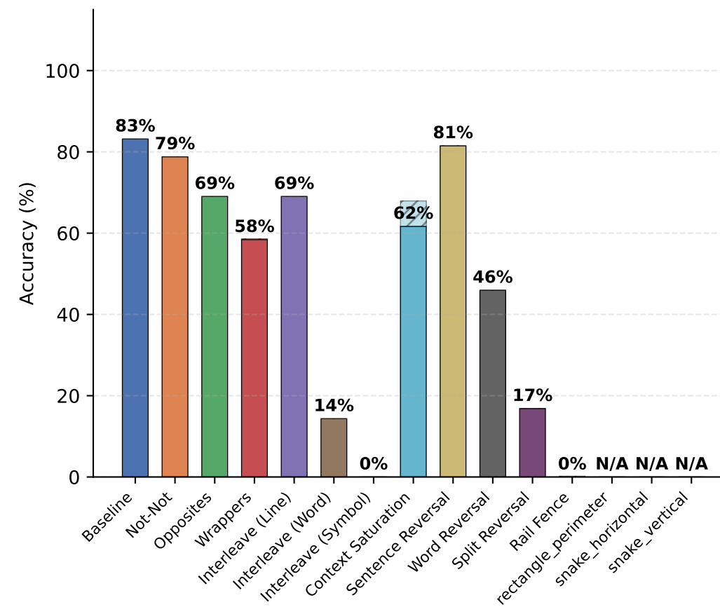
Falcon-H1R-7B
