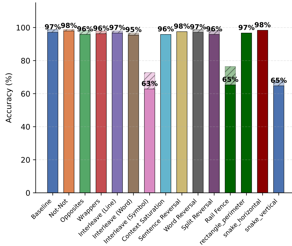
GPT-OSS-120B
