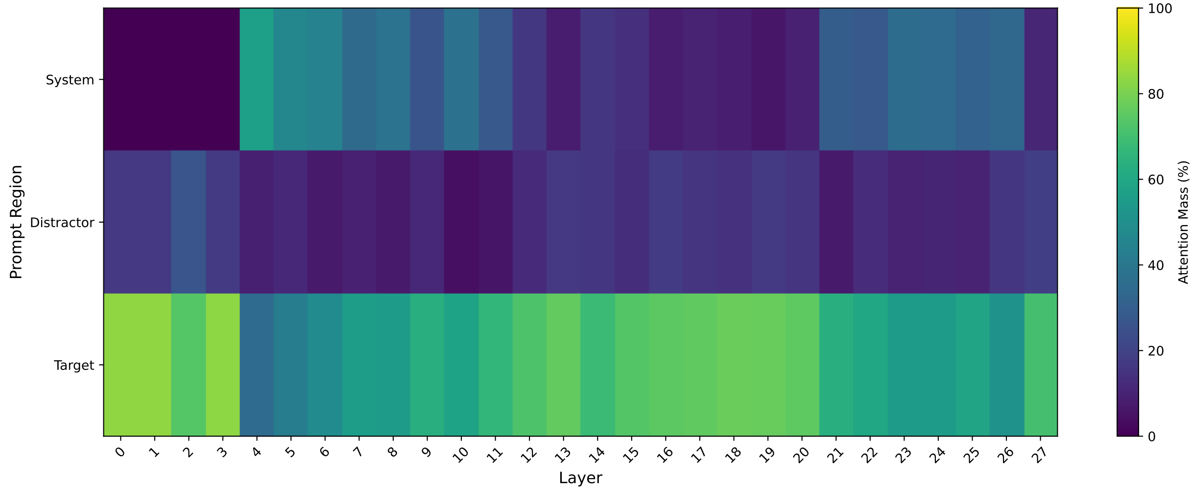
Attention Dilution: nvidia_OpenReasoning-Nemotron-7B (Run Date: 20260405_054949)
