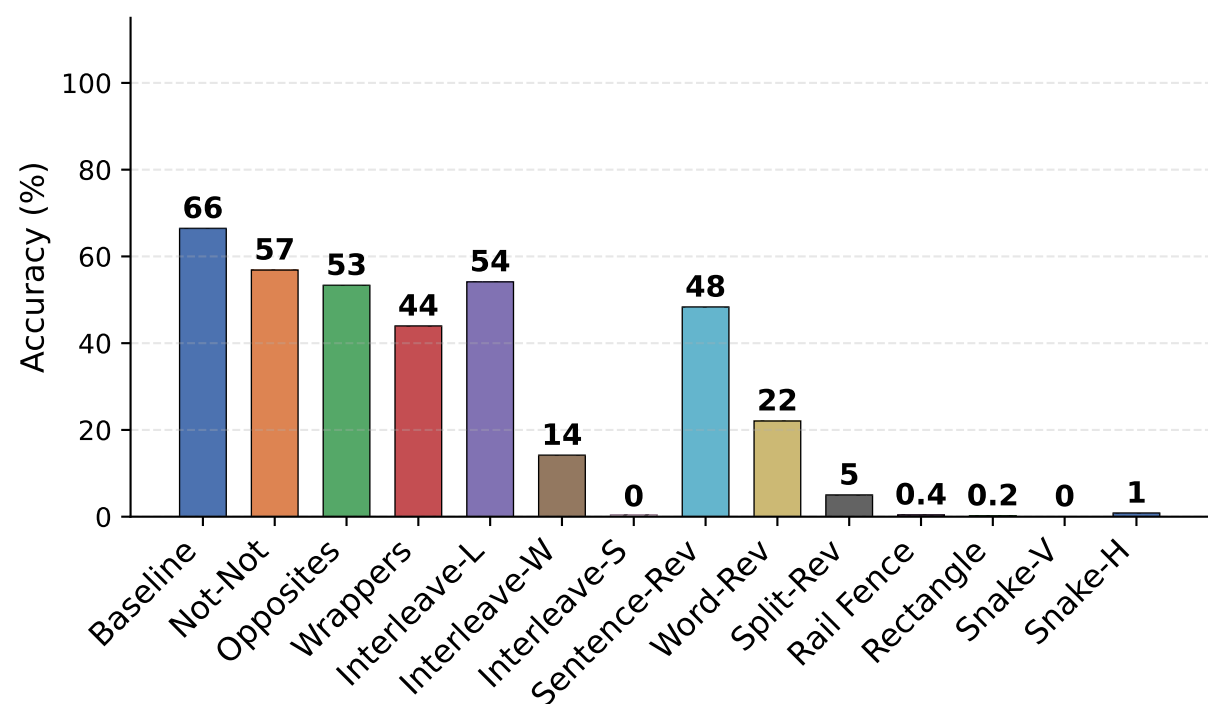
DSR1-Llama-70B
