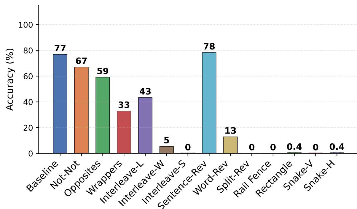
Nemotron-7B
