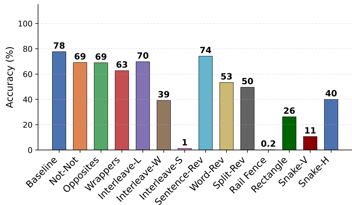
GPT-OSS-120B
