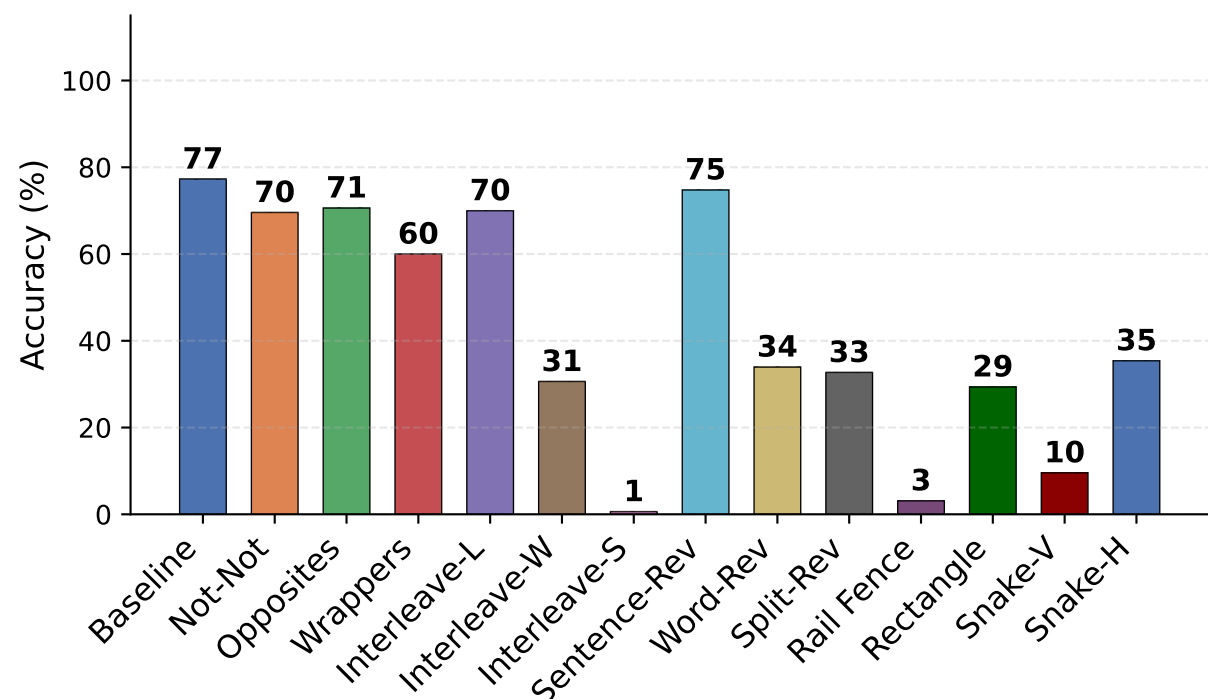
GPT-OSS-120B
