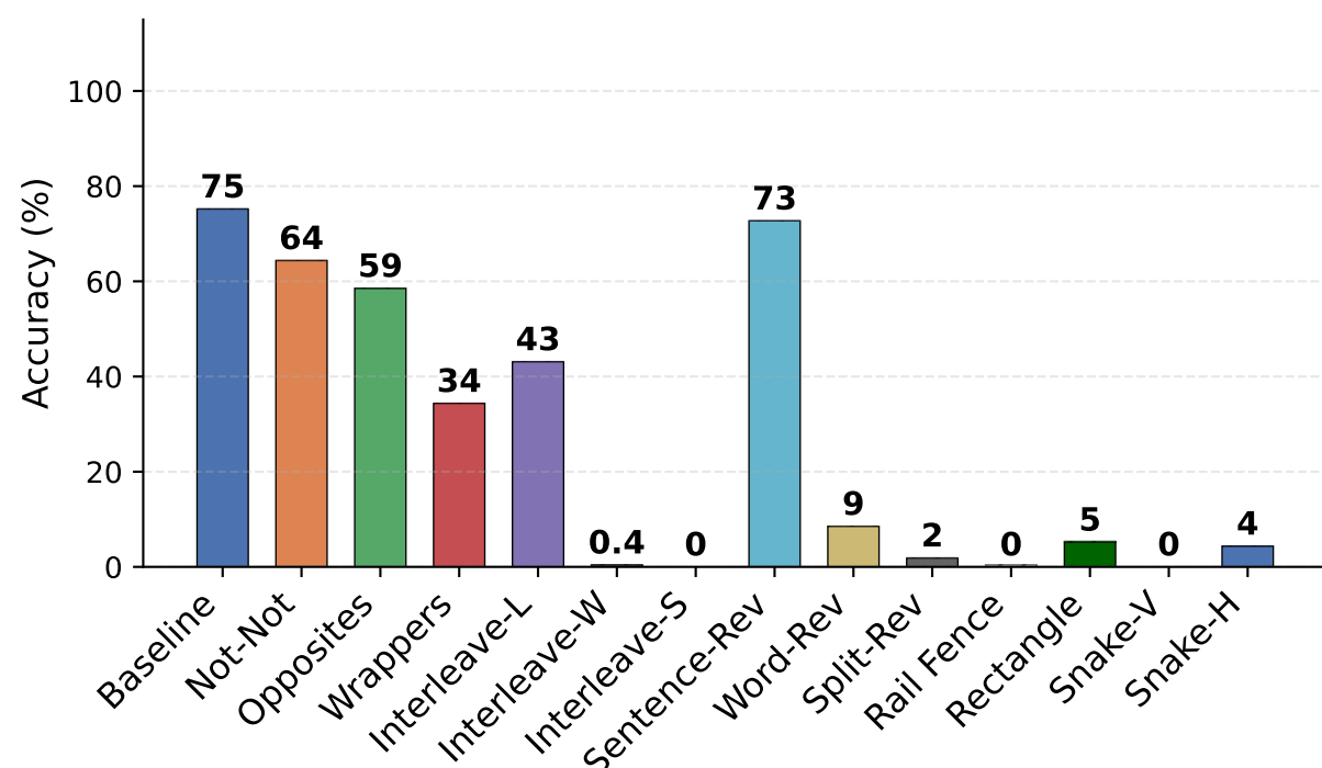
Nemotron-7B
