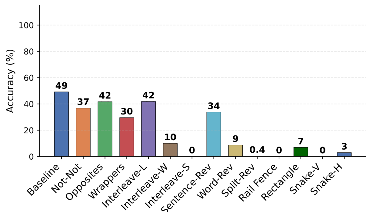
DSR1-Llama-70B
