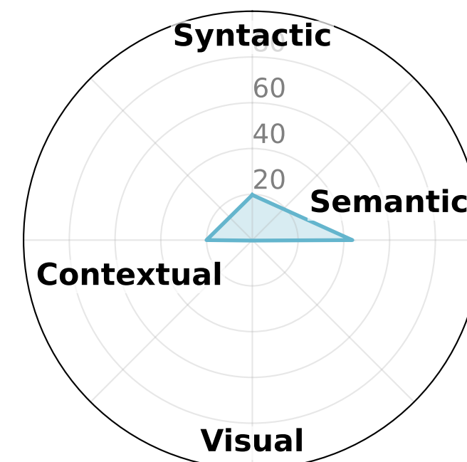
DSR1-Llama-70B
