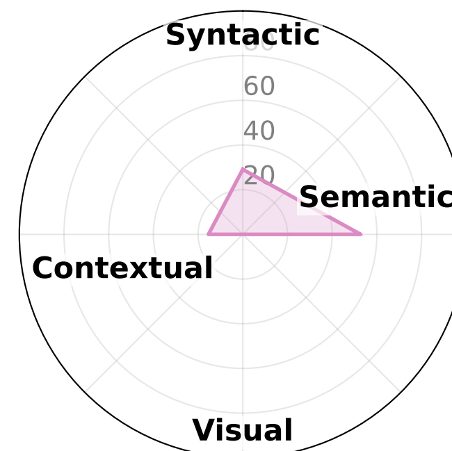
Nemotron-7B
