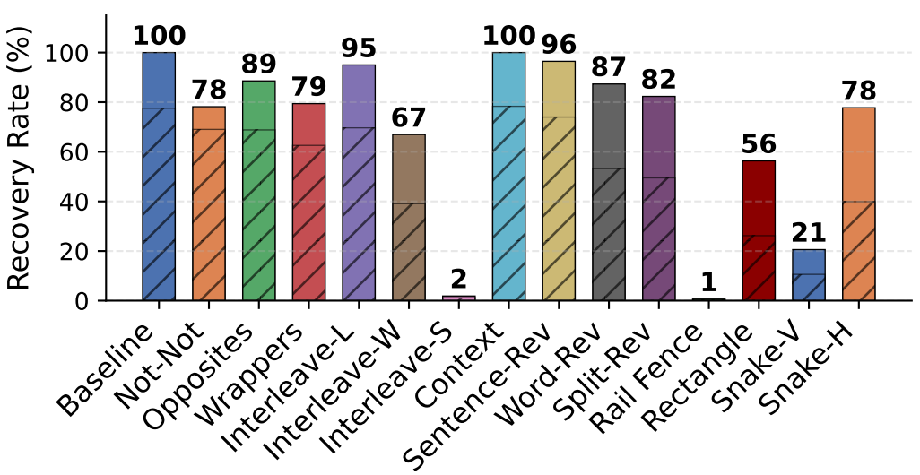
GPT-OSS-120B
