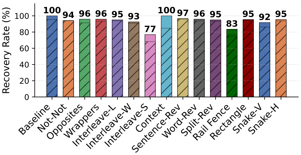
GPT-OSS-120B
