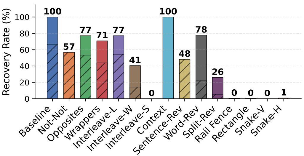
DSR1-Llama-70B
