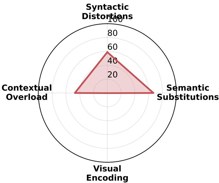
Falcon-H1R-7B
