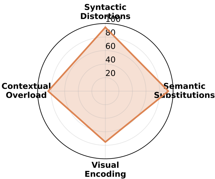
GPT-OSS-120B
