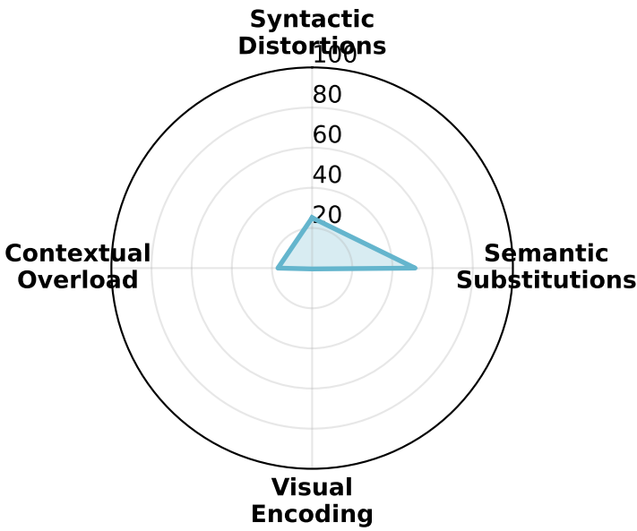
DSR1-Llama-70B
