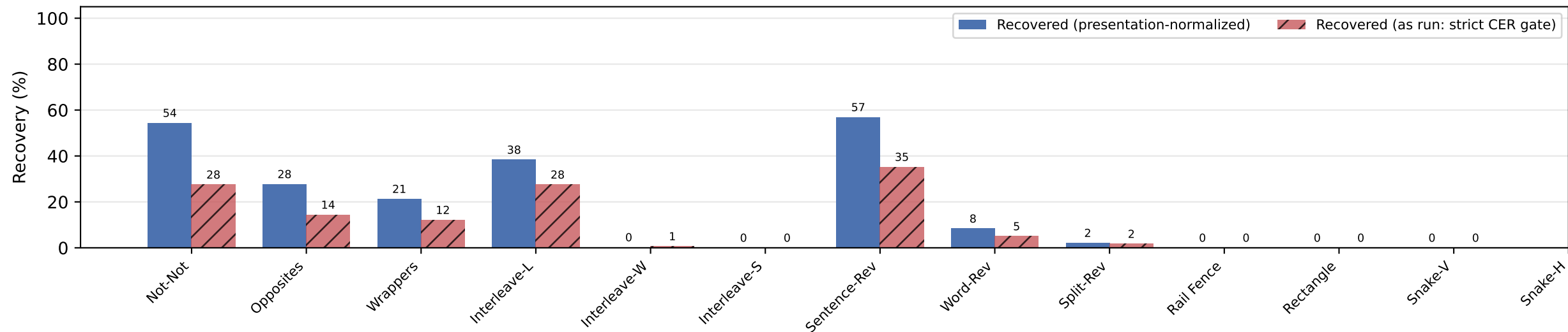
Nemotron-7B
