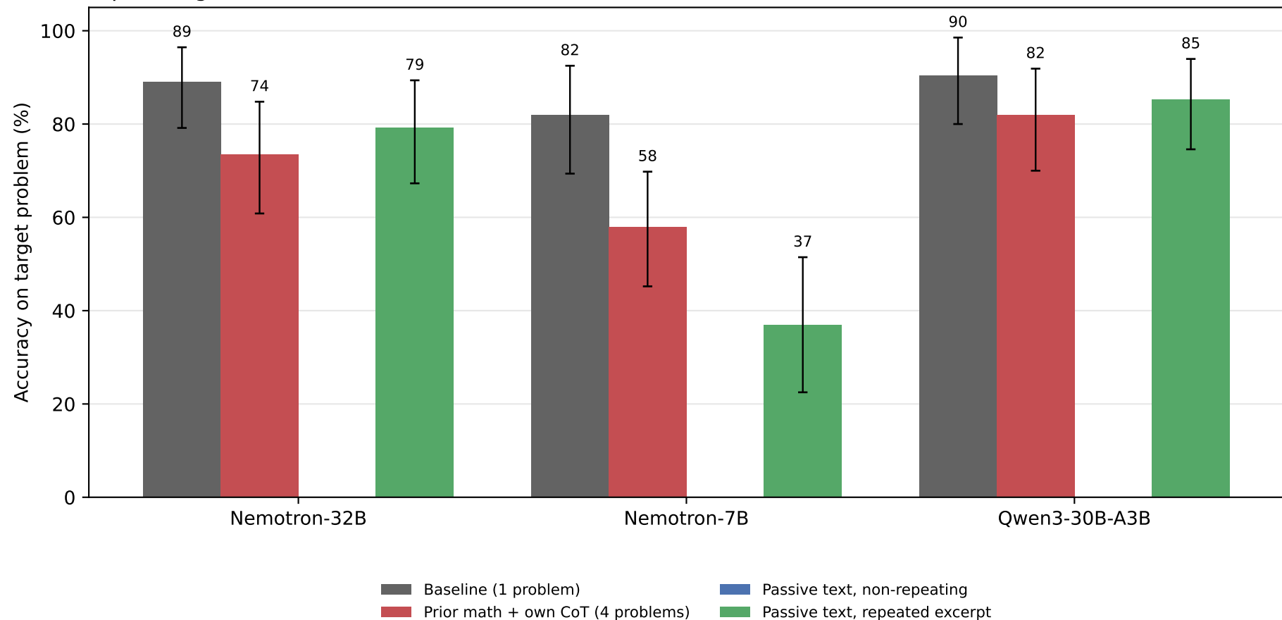
Equal-length context control — AIME 2024
