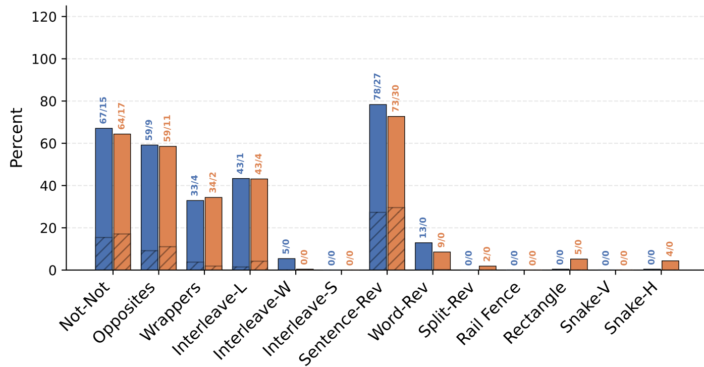
Nemotron-7B
