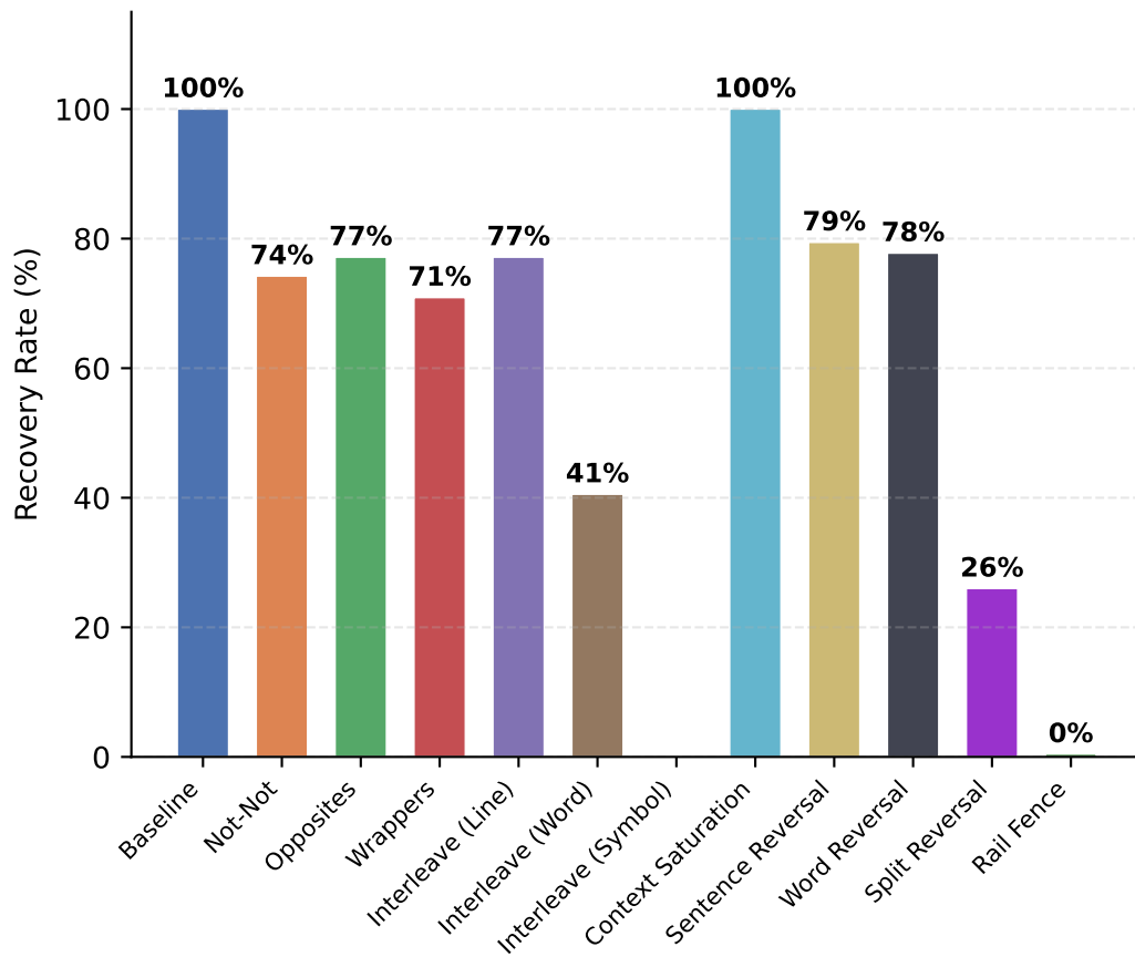
DSR1-Llama (70B)
