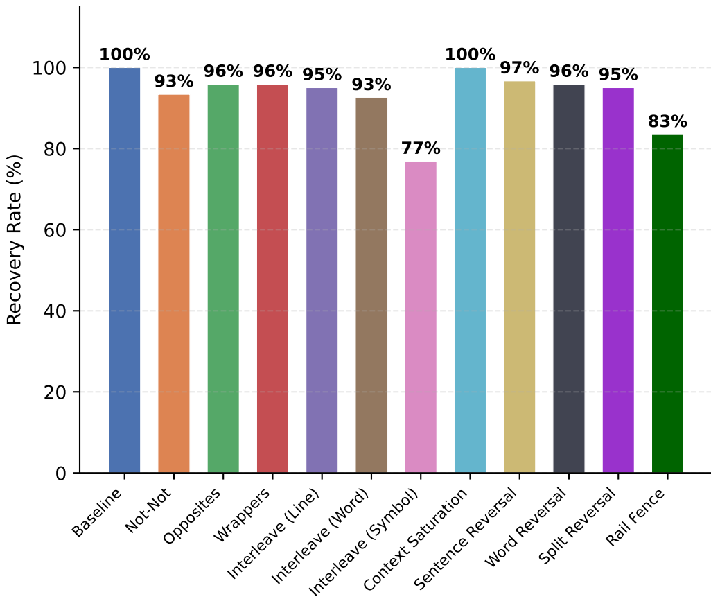
Falcon-H1R (7B)
