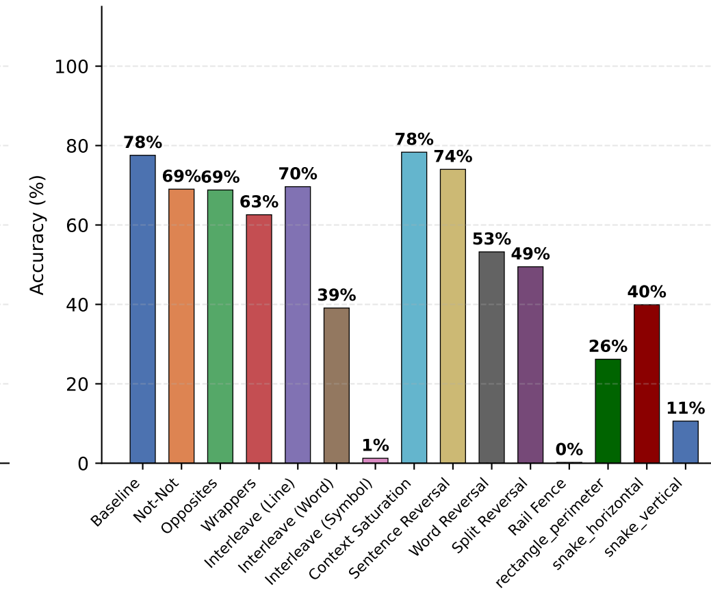
DSR1-Llama-70B
