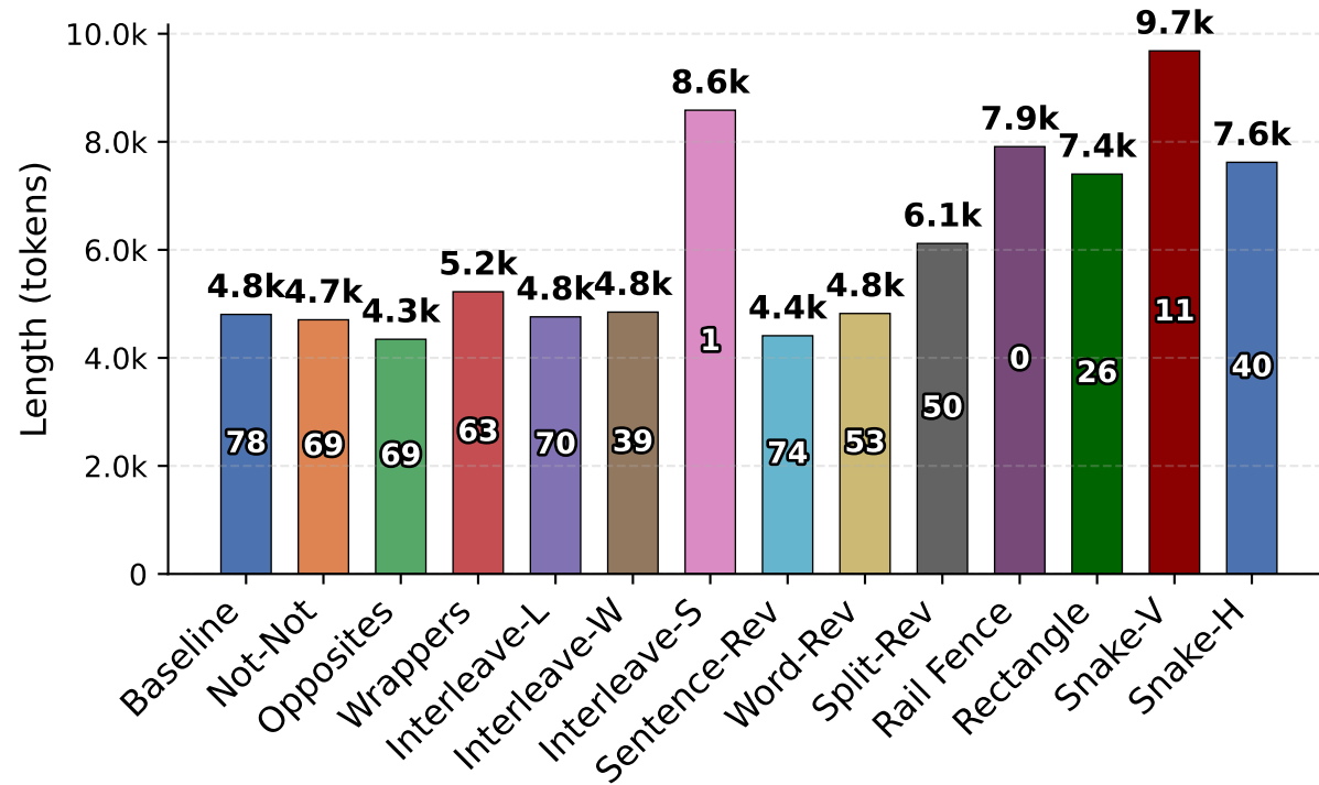
GPT-OSS-120B
