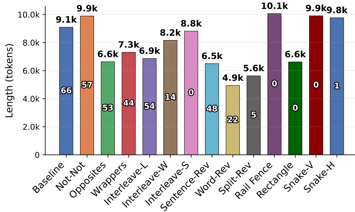
DSR1-Llama-70B
