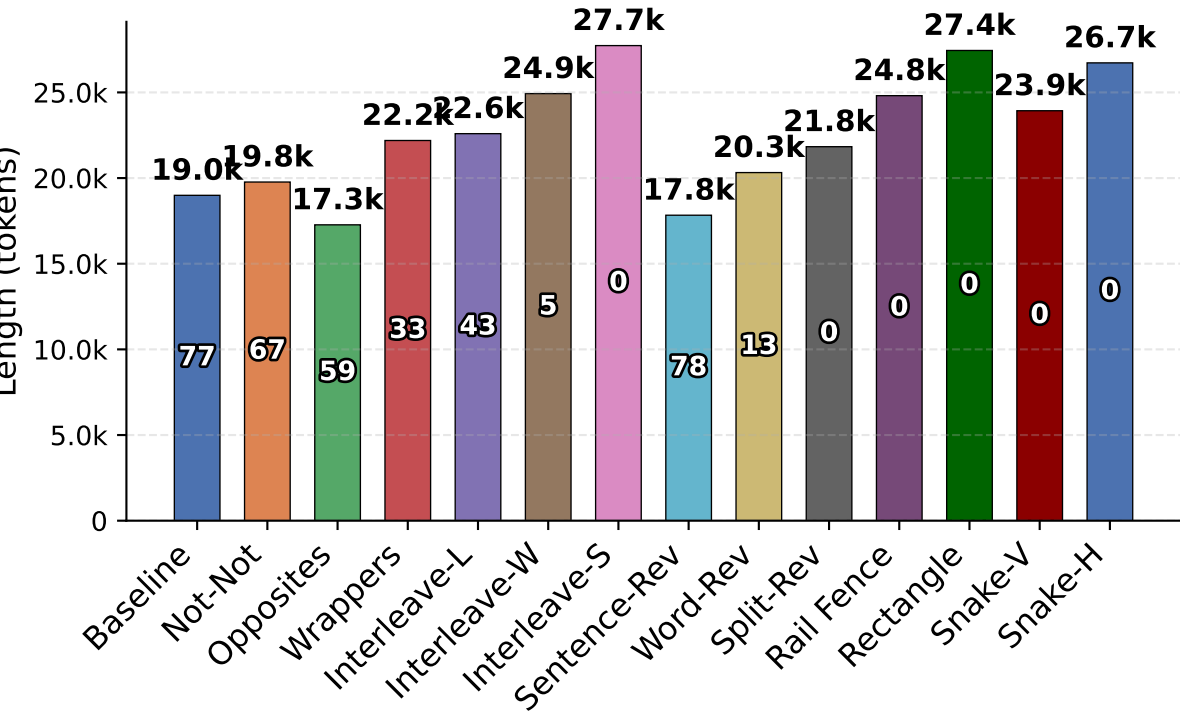
Nemotron-7B
