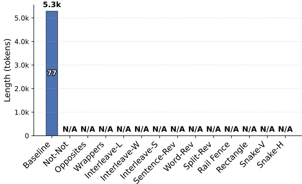
GPT-OSS-120B
