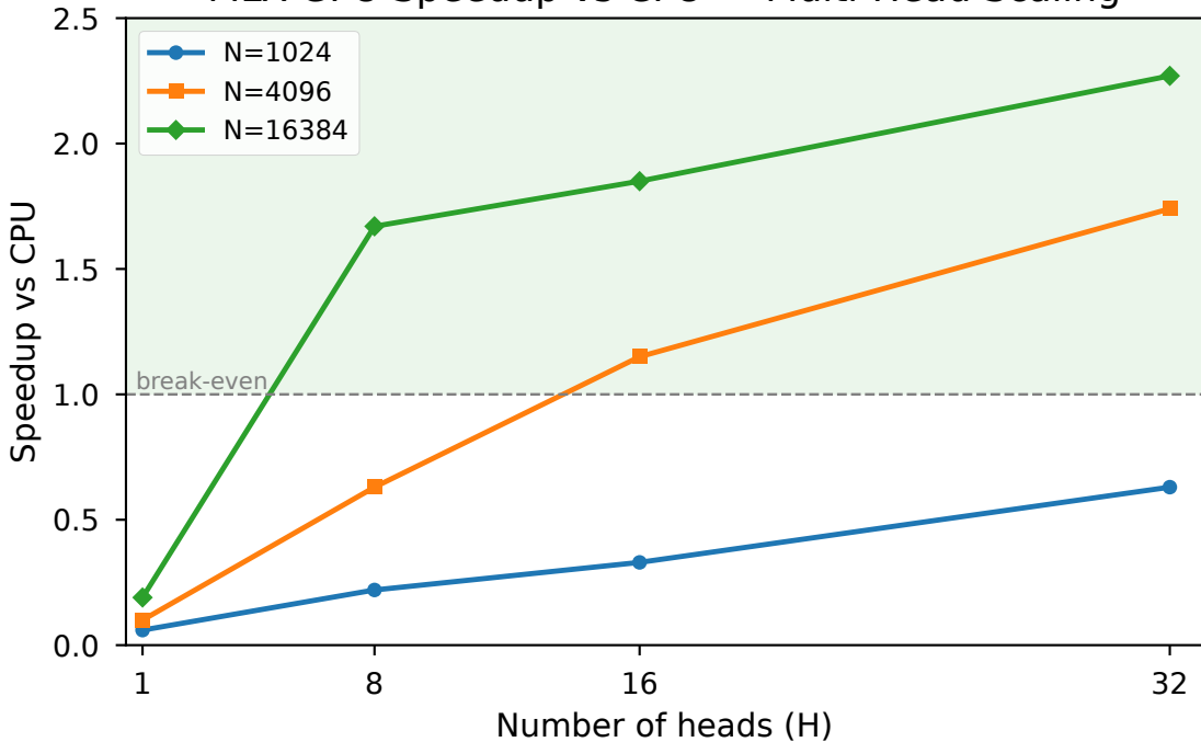
MLX GPU Speedup vs CPU — Multi-Head Scaling
