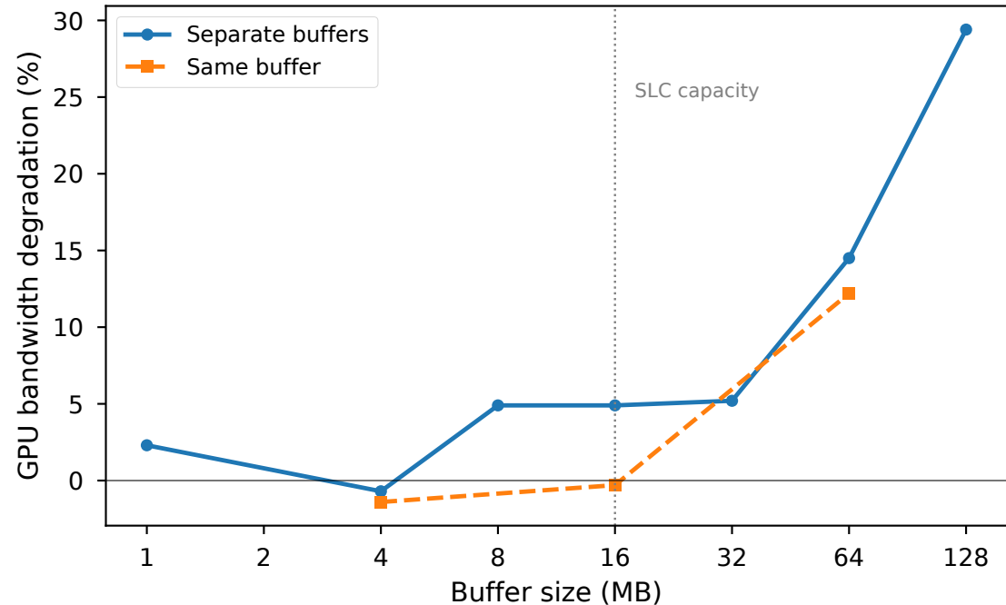
GPU Read Bandwidth Degradation Under CPU Contention
