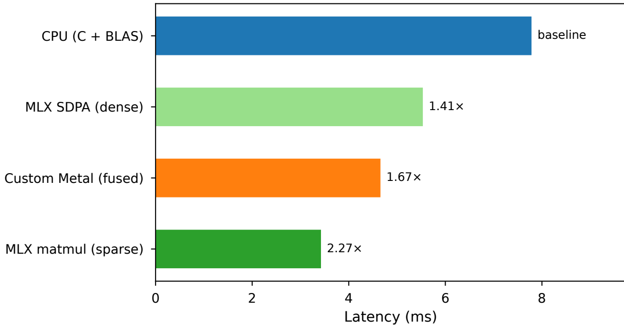
Framework Comparison — H=32, N=16K, D=128
