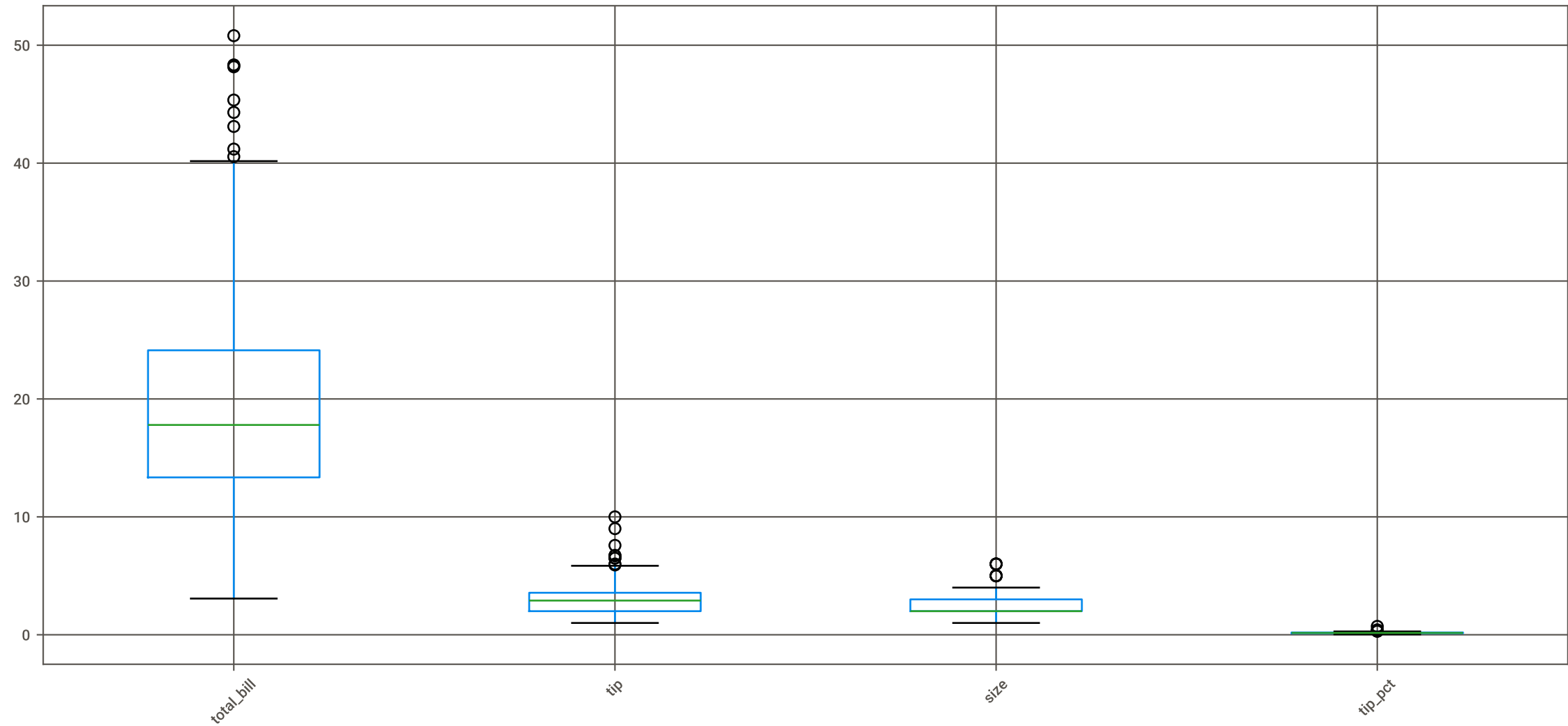
Box Plots of Numeric Variables
