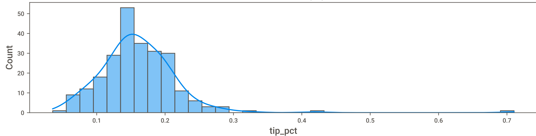
Distribution of tip_pct
