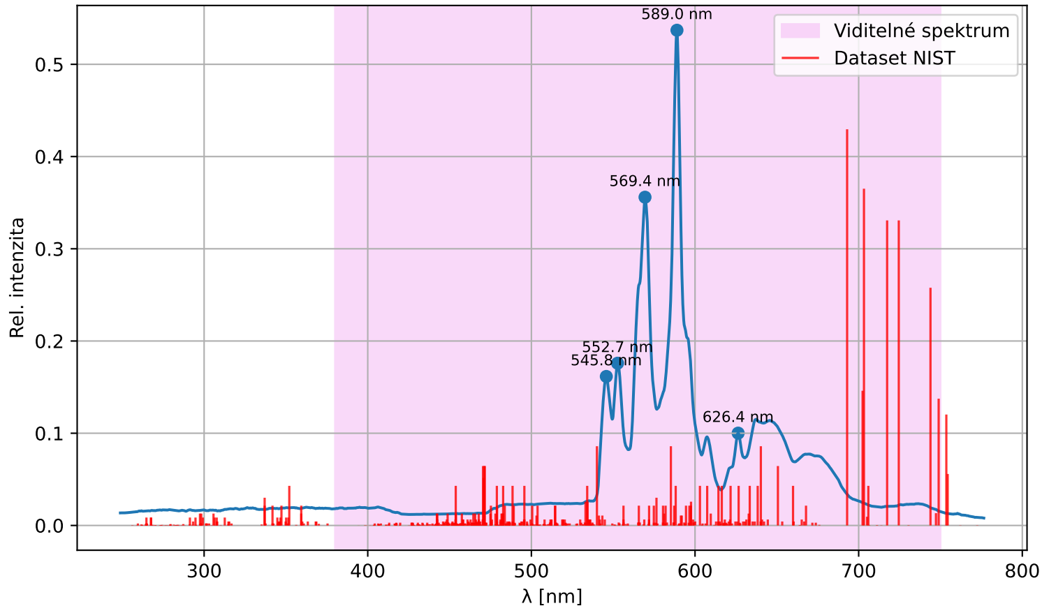
Spektrum I(\lambda) (Neon)
