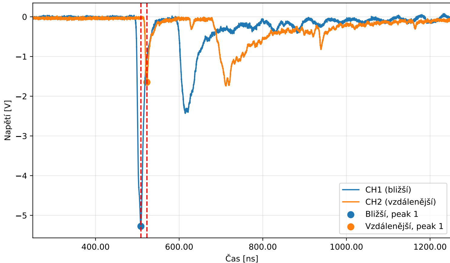
Peak #1, \Delta t = 14.330 ns
