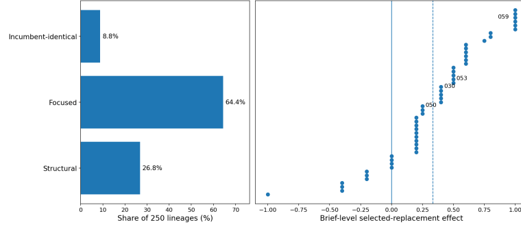
Figure 5: Competitive refinement separates whether a lineage changes from whether the adopted change helps. Left: final states over 250 lineages. Right: brief-level exact-parent effects among briefs with at least one adopted replacement, sorted by effect; the dashed line is the brief-balanced mean. Labels mark cases used later in the mechanism analysis.
