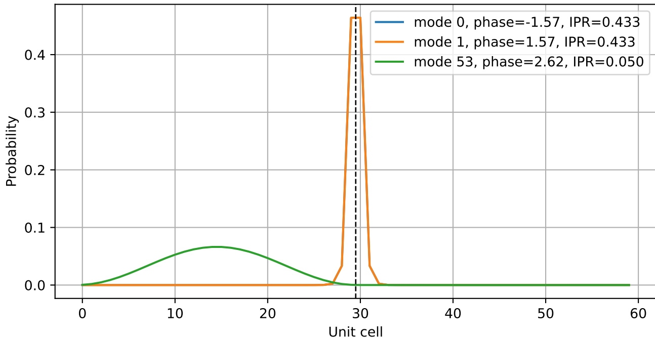
Interface modes, \theta_L = 1.05 , \theta_R = -1.05
